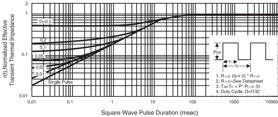
Figure 13. Normalized Thermal Transient Impedance Curve
