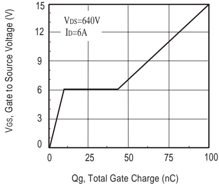
Figure 9. Gate Charge
