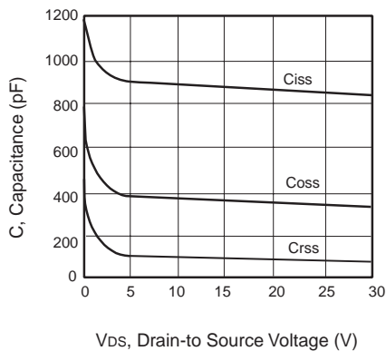
Figure 3. Capacitance
