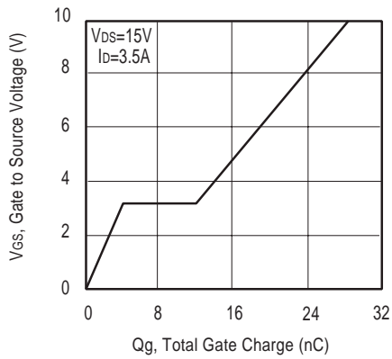
Figure 9. Gate Charge
