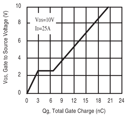
Figure 9. Gate Charge
