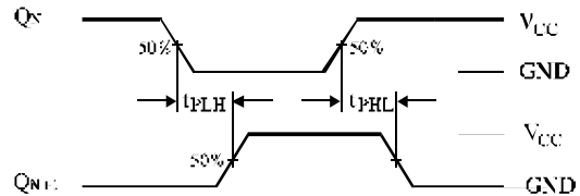
Figure 2. Switching Waveforms
