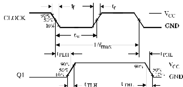
Figure 1. Switching Waveforms
