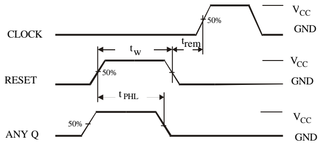
Figure 3. Switching Waveforms
