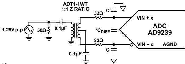
Figure 47. Differential Transformer-Coupled Configuration for Baseband Applications
