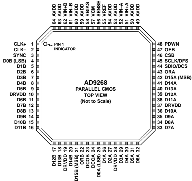
Figure 6. LFCSP Parallel CMOS Pin Configuration (Top View)
