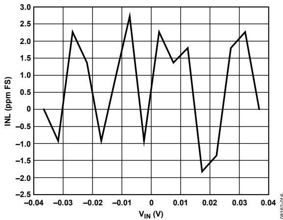
Figure 16. Integral Nonlinearity ( V_{REF} = AV_{DD} , Gain = 128)
