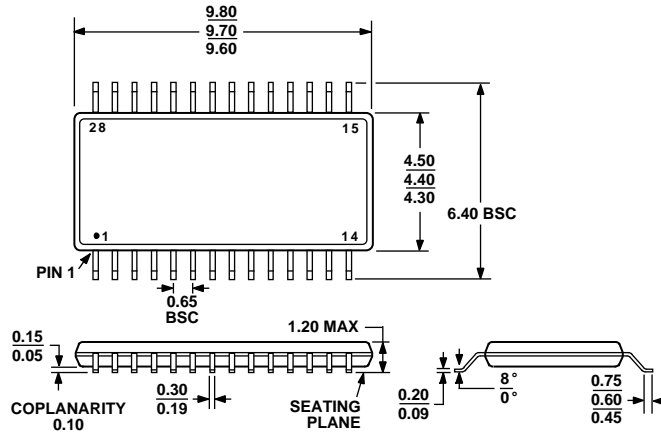
Figure 69. 28-Lead Thin Shrink Small Outline Package [TSSOP] (RU-28)
