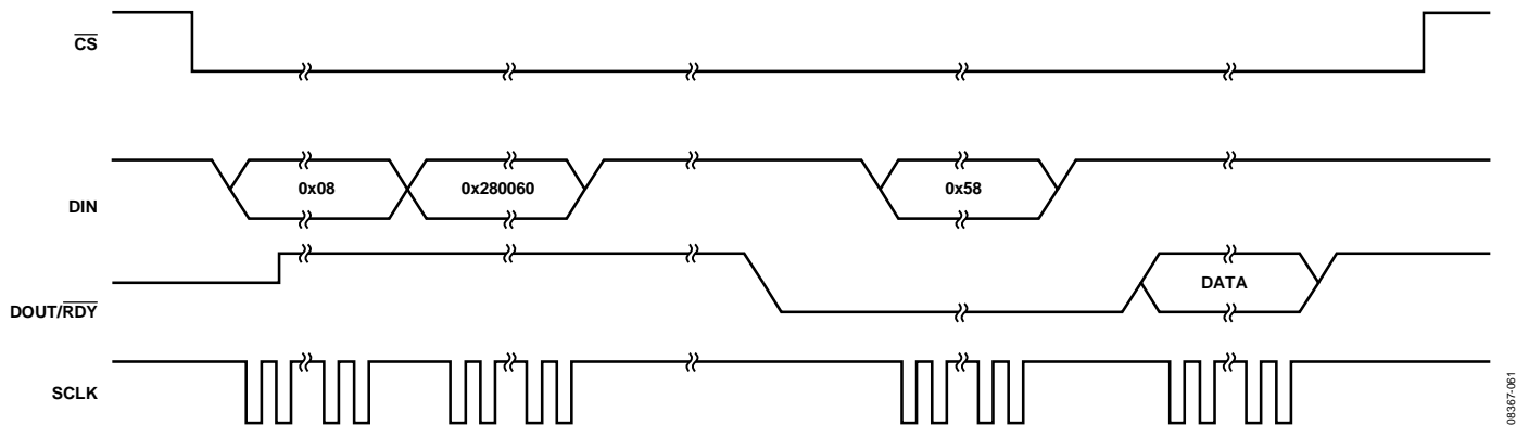
Figure 25. Single Conversion
