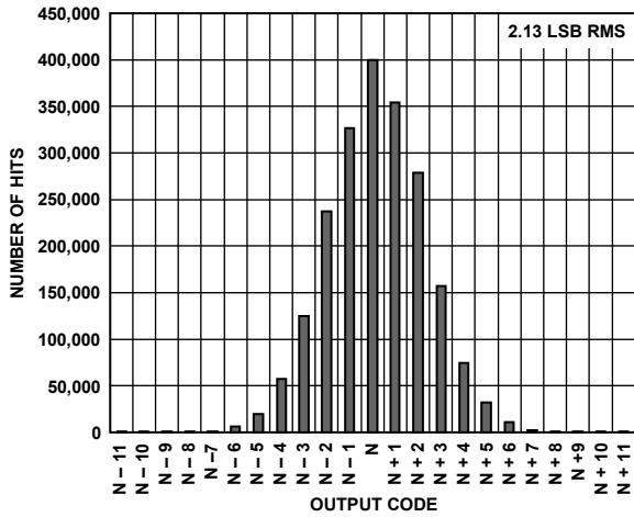
Figure 49. AD9265-125 Grounded Input Histogram
