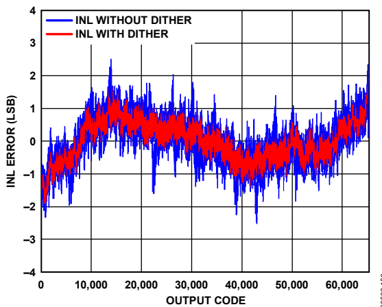
Figure 50. AD9265-125 INL with f_{IN} = 9.7 MHz
