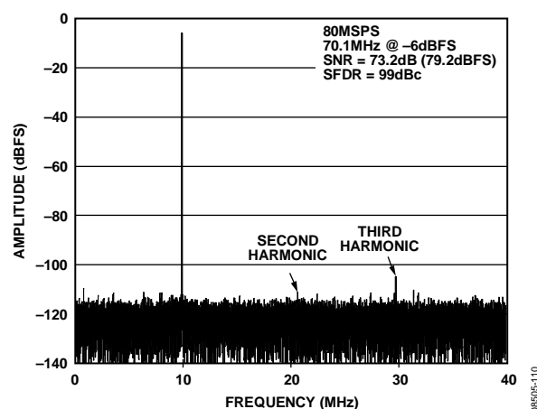
Figure 10. AD9255-80 Single-Tone FFT with f_{IN} = 70.1 MHz @ -6 dBFS with Dither Enabled
