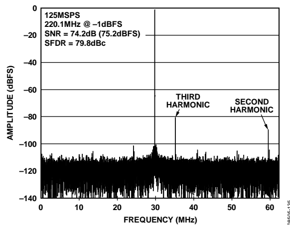
Figure 35. AD9255-125 Single-Tone FFT with f_{IN} = 220.1 MHz
