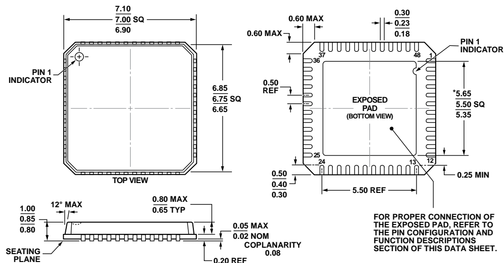
Figure 85. 48-Lead Lead Frame Chip Scale Package [LFCSP_VQ] 7 mm × 7 mm Body, Very Thin Quad (CP-48-8)
