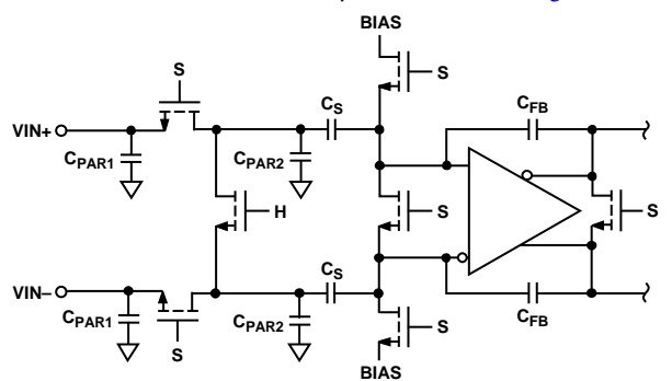
Figure 64. Switched-Capacitor Input
