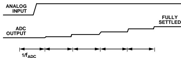
Figure 29. Asynchronous Step Change in Analog Input
