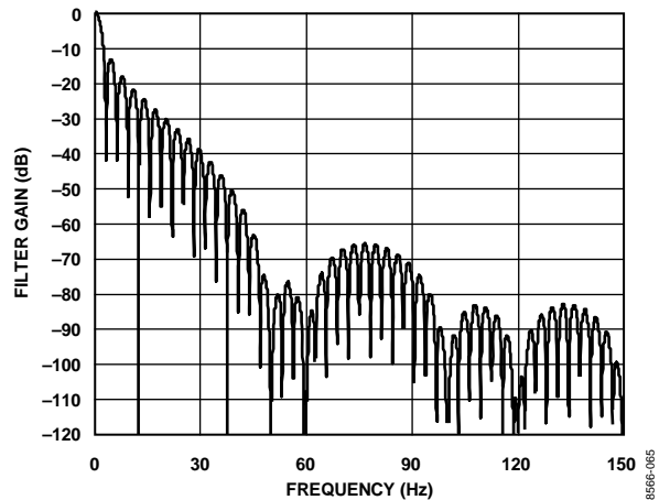
Figure 66. Filter Response for Average + Decimate Filter (Sinc 3 Filter, FS[9:0] = 96, Average by 16)
