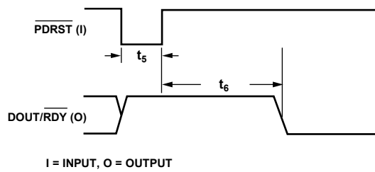
Figure 4. Resetting the AD7170
