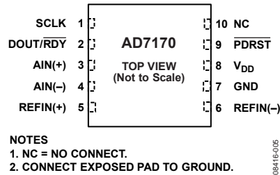
Figure 5. Pin Configuration
