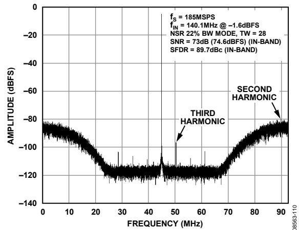
Figure 10. Single-Tone FFT with f_{IN} = 140.1\text{ MHz} , NSR Enabled in 22% BW Mode with Tuning Word = 28
