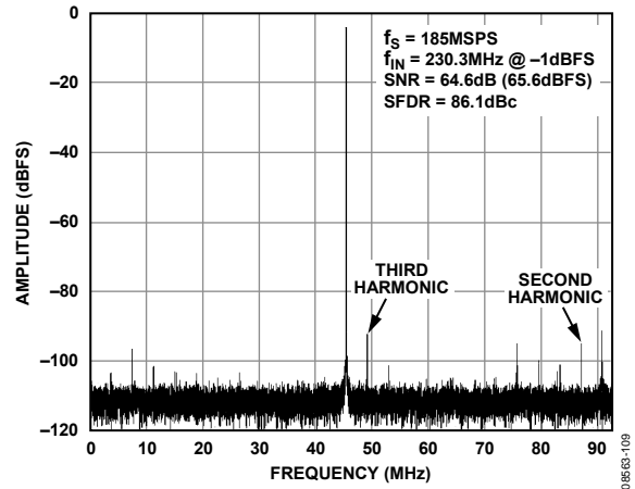
Figure 9. Single-Tone FFT with f_{IN} = 230.3\text{ MHz}
