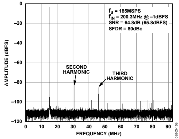
Figure 8. Single-Tone FFT with f_{IN} = 200.3\text{ MHz}
