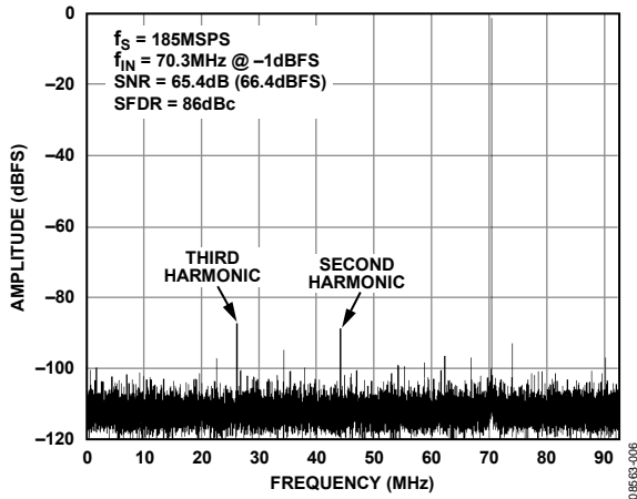
Figure 6. Single-Tone FFT with f_{IN} = 70.3\text{ MHz}
