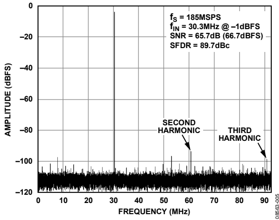
Figure 5. Single-Tone FFT with f_{IN} = 30.3\text{ MHz}
