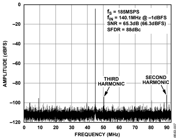
Figure 7. Single-Tone FFT with f_{IN} = 140.1\text{ MHz}
