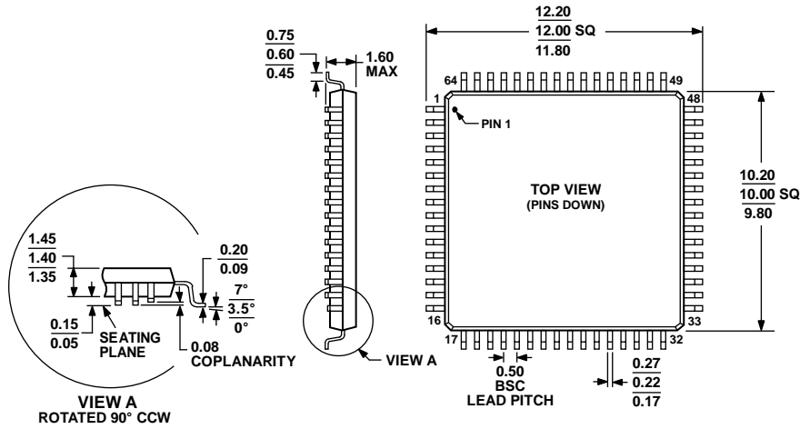
Figure 65. 64-Lead Low Profile Quad Flat Package [LQFP] (ST-64-2)
