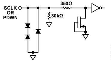
Figure 45. Equivalent SCLK or PDWN Input Circuit
