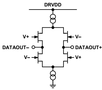
Figure 41. Equivalent LVDS Output Circuit
