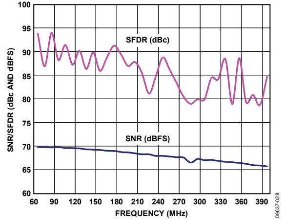
Figure 21. AD9613-210 Single-Tone SNR/SFDR vs. Input Frequency ( f_{IN} )
