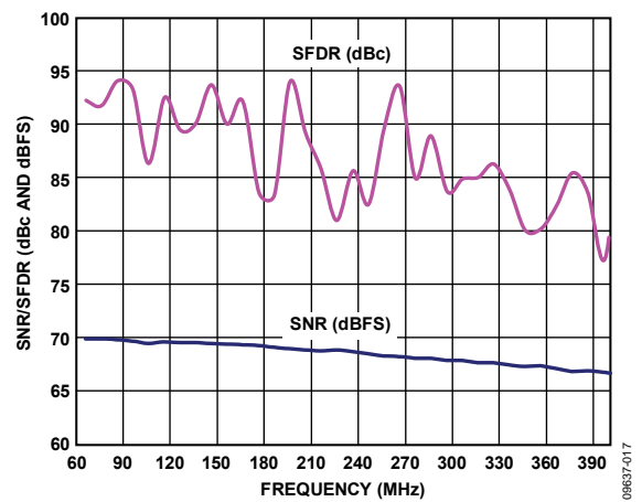
Figure 10. AD9613-170 Single-Tone SNR/SFDR vs. Input Frequency ( f_{IN} )
