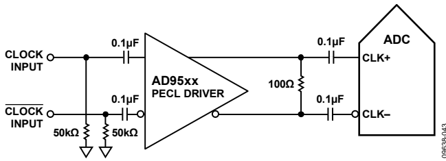
Figure 36. Differential LVDS Sample Clock (Up to 625 MHz)
