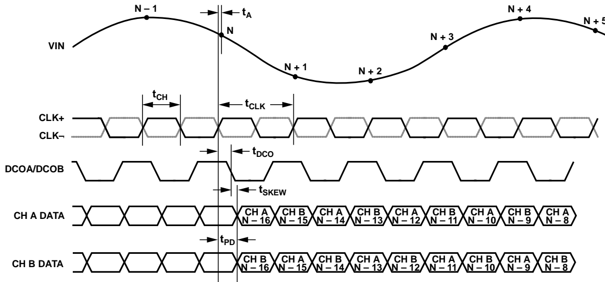
Figure 3. CMOS Interleaved Output Mode Data Output Timing
