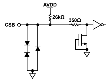
Figure 45. Equivalent CSB Input Circuit
