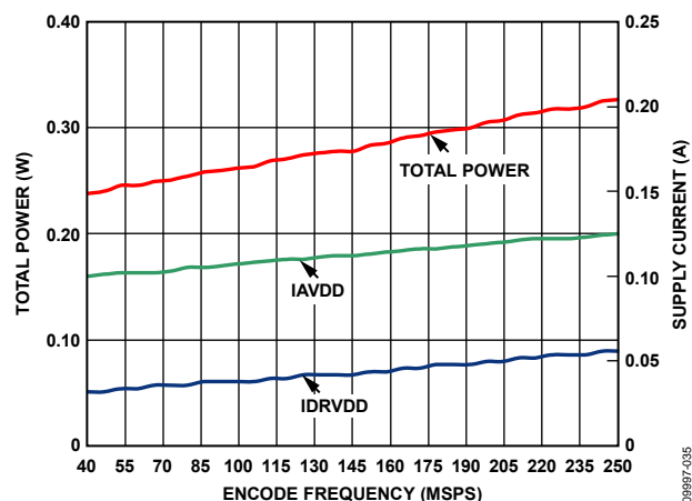
Figure 35. AD6672-250 Power and Current vs. Sample Rate
