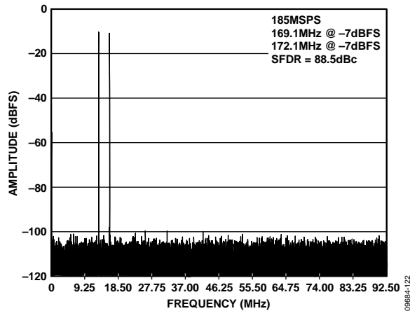
Figure 22. Two Tone FFT, f_{IN1} = 169.1 MHz and f_{IN2} = 172.1 MHz
