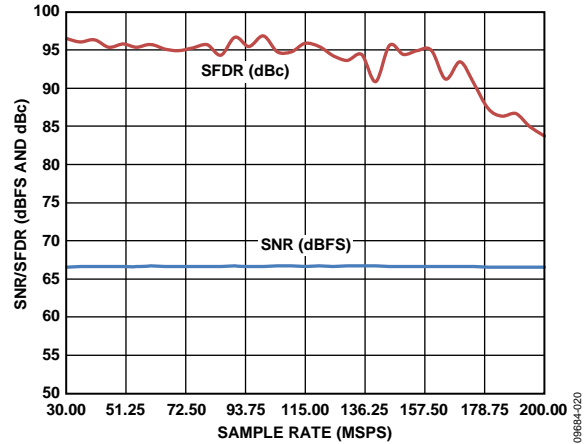
Figure 20. Single Tone SNR/SFDR vs. Sample Rate ( f_s ), f_{IN} = 70.3 MHz
