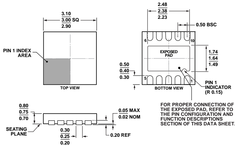
Figure 45. 10-Lead Lead Frame Chip Scale Package [QFN (LFCS P _WD)] 3 mm × 3 mm Body, Very Very Thin, Dual Lead (CP-10-9)
