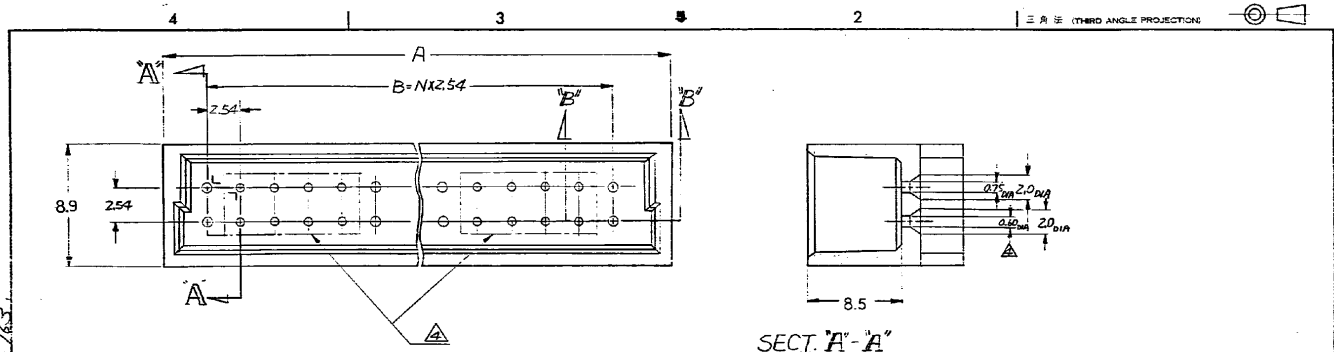
SECT. "A"-A"
