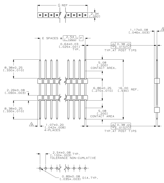
RECOMMENDED HOLE LAYOUT
