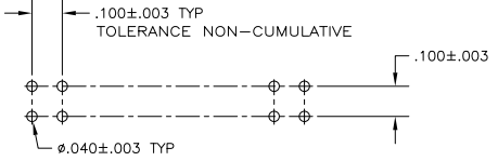
RECOMMENDED HOLE LAYOUT
