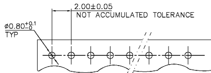
RECOMMENDED PCB LAYOUT (PCB THK=1.0~1.6)
