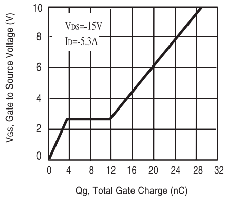
Figure 9. Gate Charge
