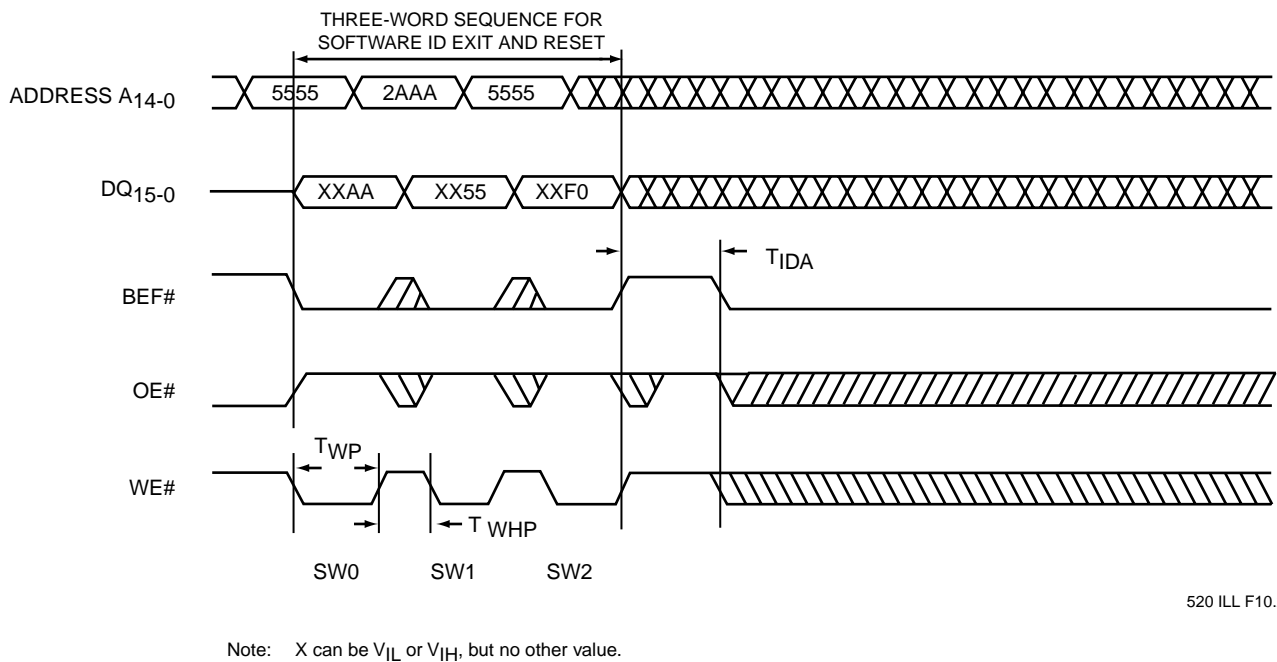
FIGURE 15: SOFTWARE ID EXIT AND RESET
