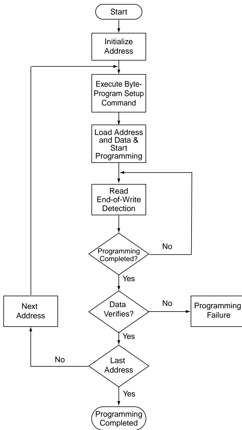
FIGURE 16: BYTE-PROGRAM FLOWCHART
