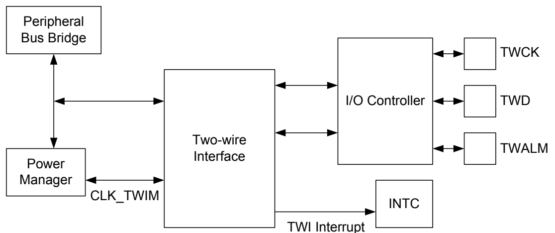
Figure 27-1. Block Diagram
