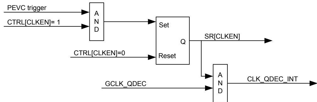
Figure 34-3. Clock Control
