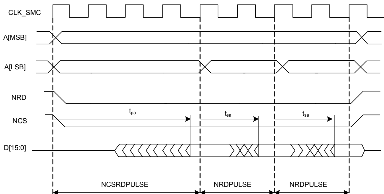
Figure 18-33. Page Mode Read Protocol (Address MSB and LSB Are Defined in Table 18-6 on page 336 )
