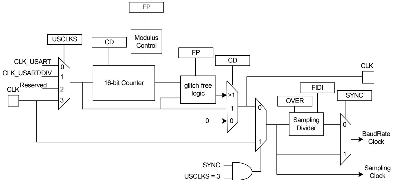
Figure 25-3. Fractional Baud Rate Generator
