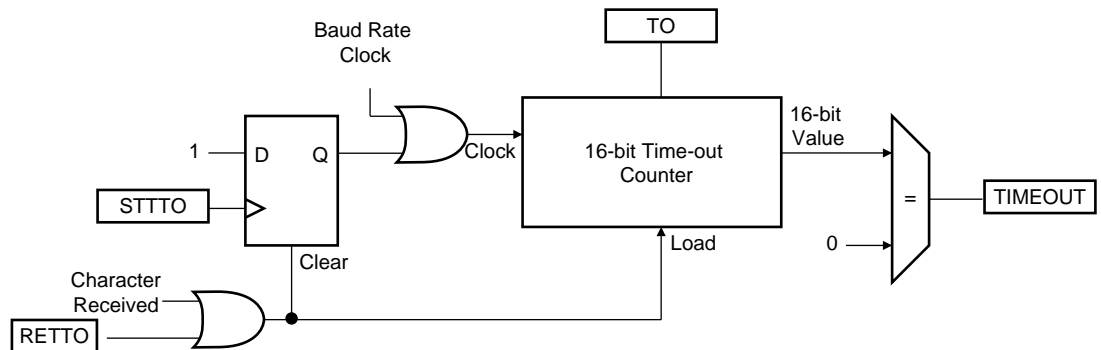
Figure 25-23. Receiver Time-out Block Diagram
