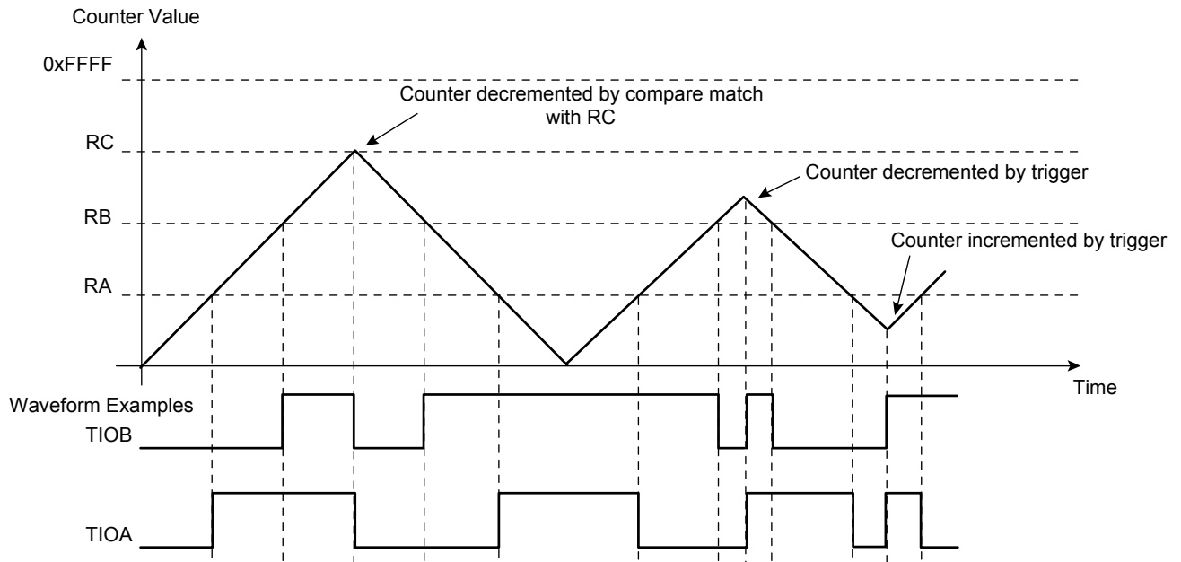
Figure 31-13. WAVSEL = 3 With Trigger
