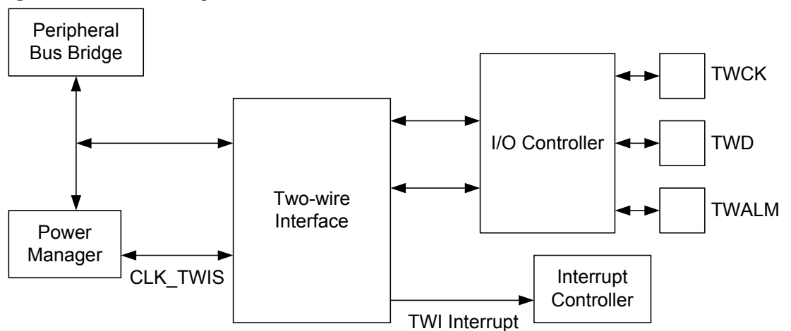
Figure 28-1. Block Diagram
