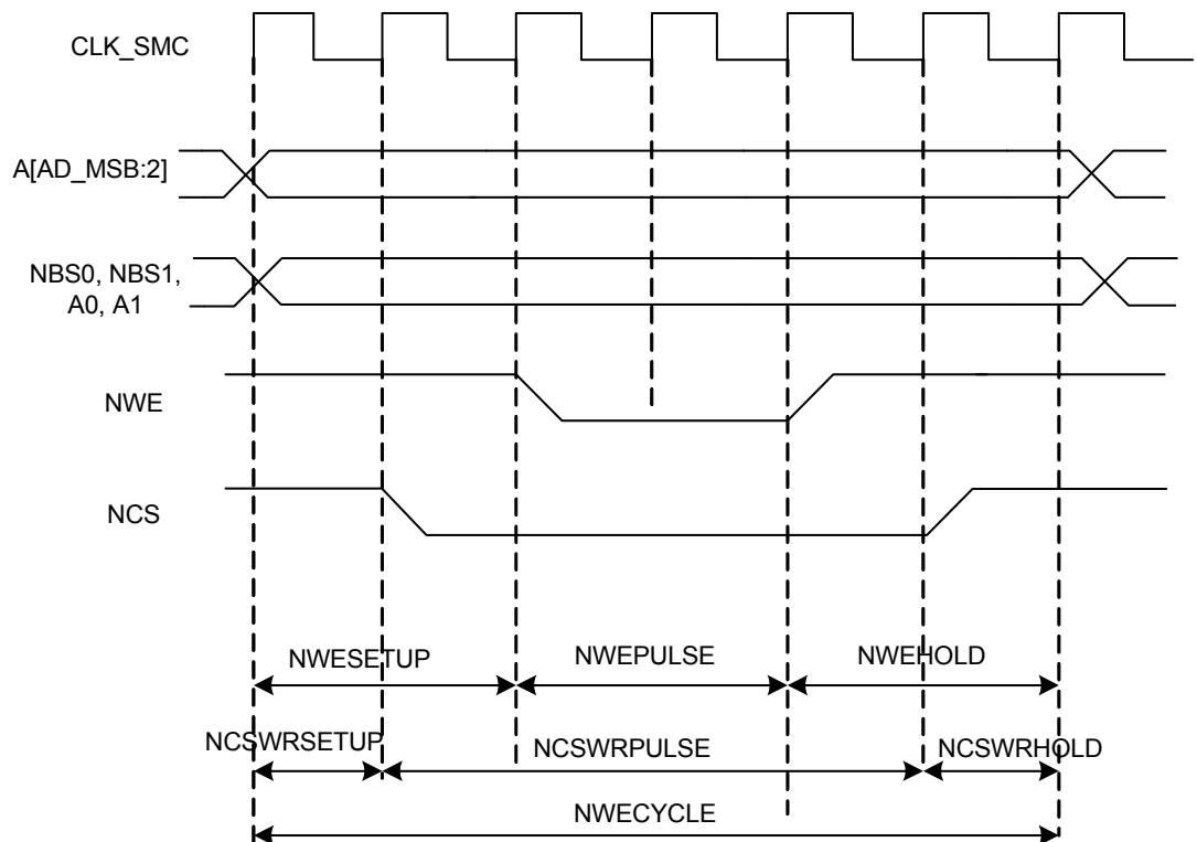
Figure 18-11. Write Cycle
