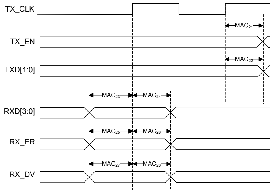
Figure 40-21. Ethernet MAC RMII Mode
