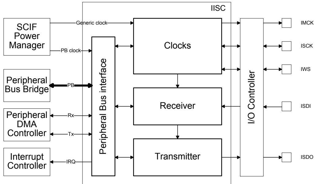
Figure 30-1. IISC Block Diagram
