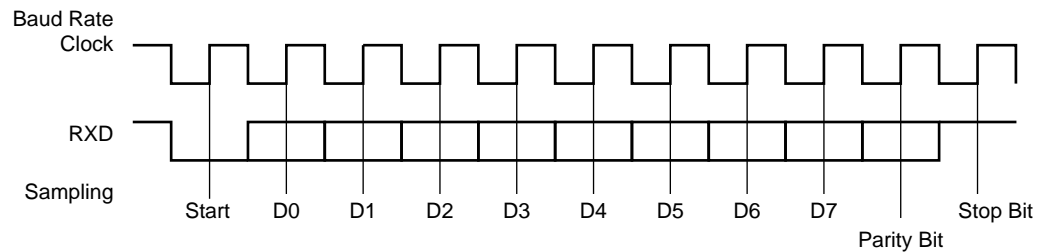
Figure 25-19. Synchronous Mode Character Reception
