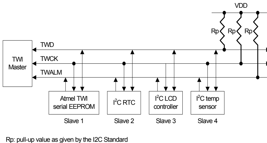
Figure 27-2. Application Block Diagram
