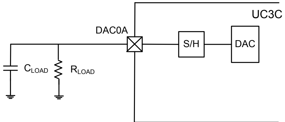
Figure 40-4. DAC output
