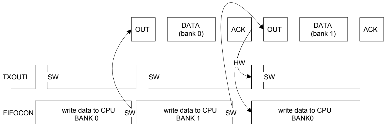
Figure 32-23. Example of an OUT pipe with two data banks and a bank switching delay
