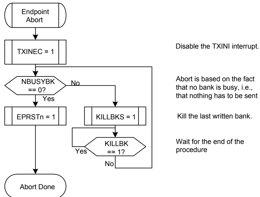
Figure 32-13. Abort Algorithm
