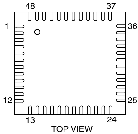
Figure 4-6. Orientation of the 48-lead QFN Package
