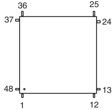
Figure 4-5. Orientation of the 48-lead LQFP Package
