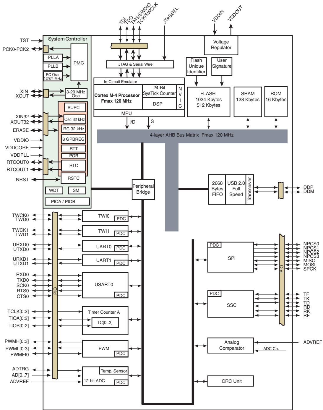
Figure 2-3. SAM4S Series 48-pin version Block Diagram
