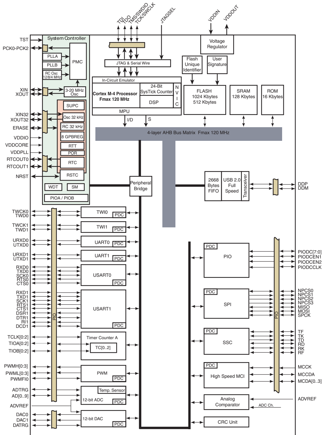
Figure 2-2. SAM4S Series 64-pin version Block Diagram
