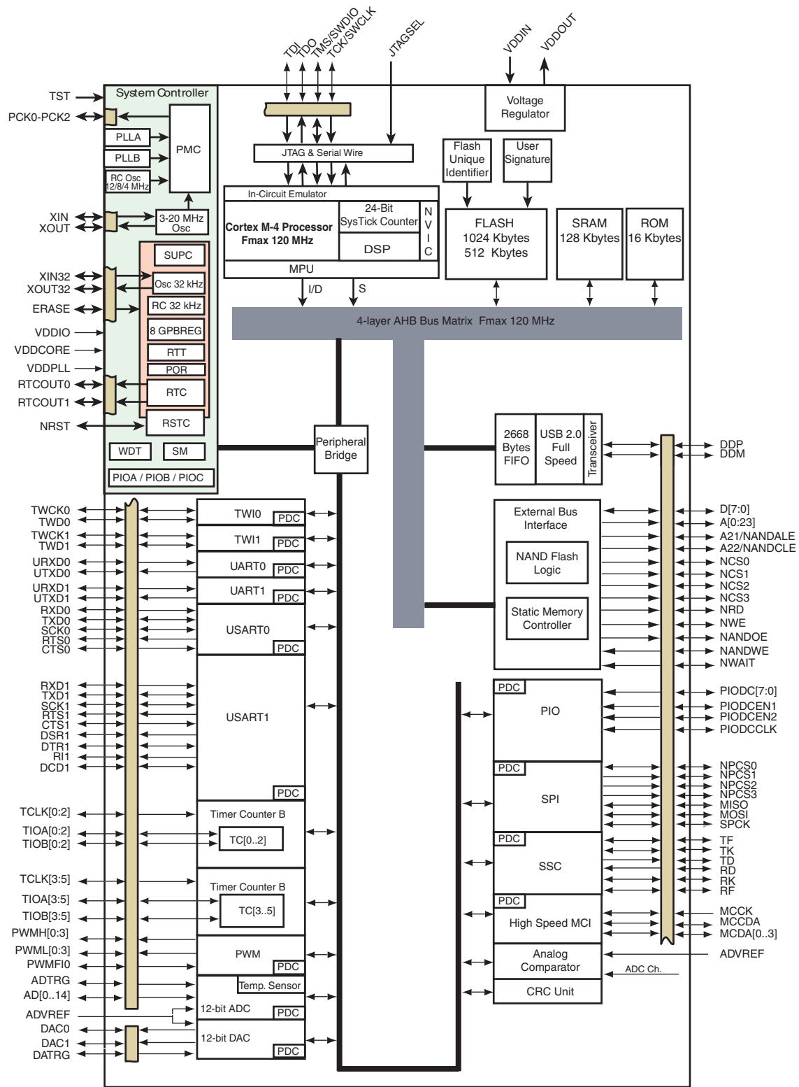
Figure 2-1. SAM4S Series100-pin version Block Diagram
