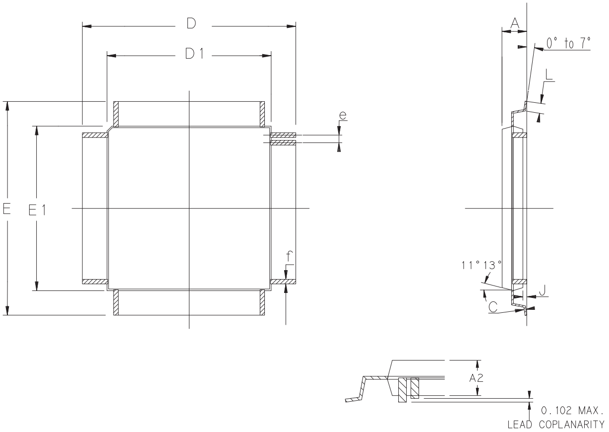
Figure 12-5. 48-lead LQFP Package Mechanical Drawing
