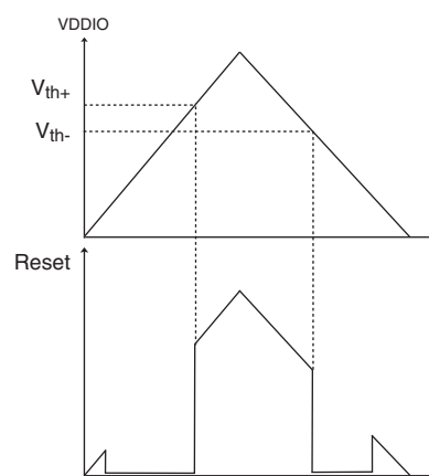
Figure 43-3. Zero-Power-on Reset Characteristics
