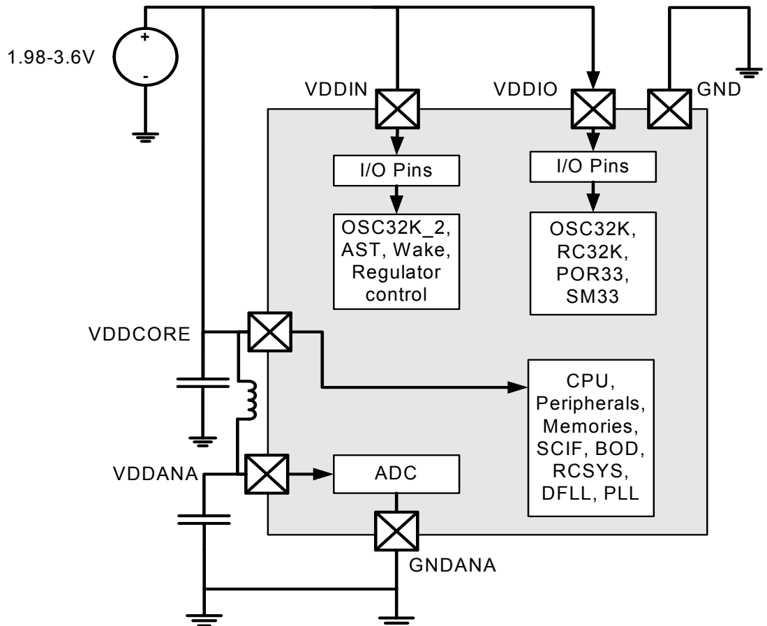
Figure 5-3. 1.8V Single Supply Mode
