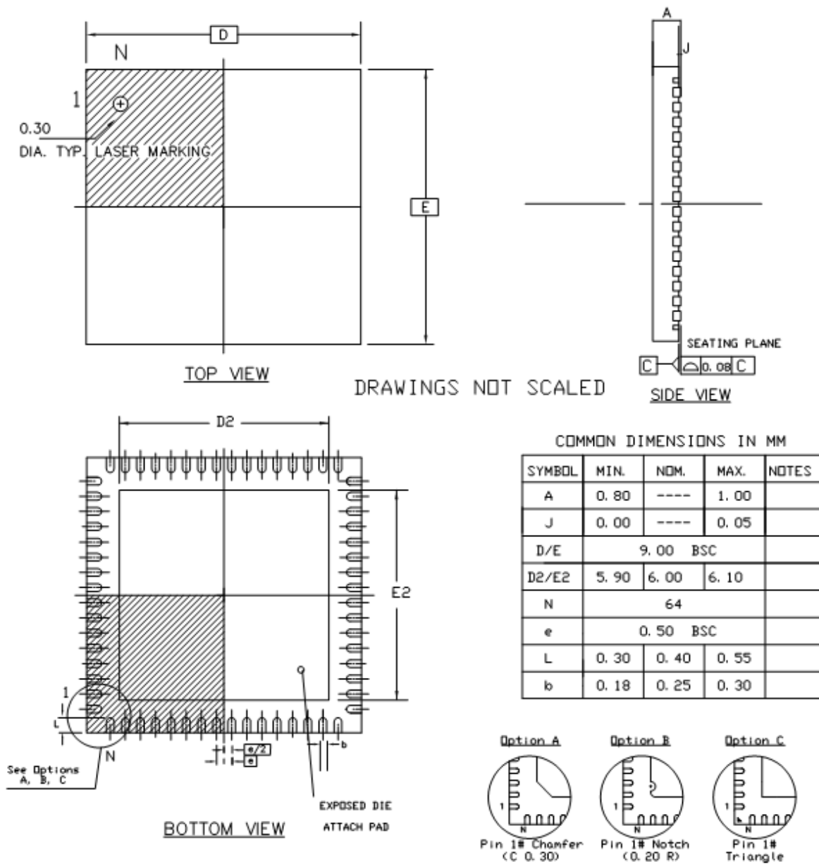
Figure 8-5. QFN-64 Package Drawing
