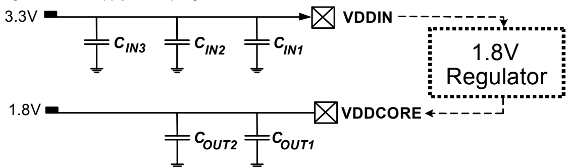
Figure 5-1. Supply Decoupling.
