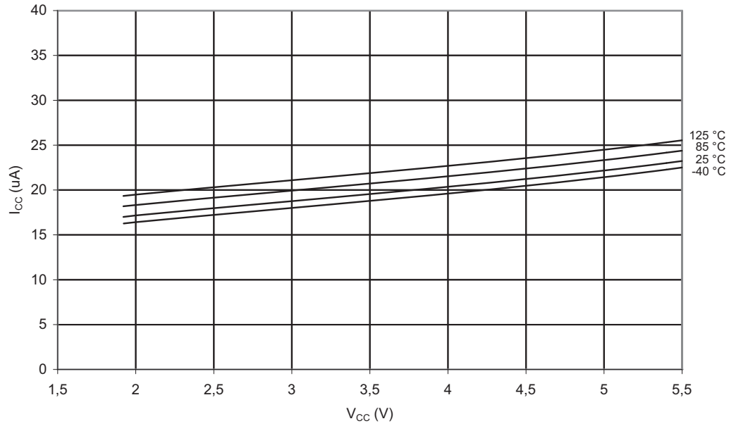
Figure 2-10. Programming Current vs. V_{CC}
