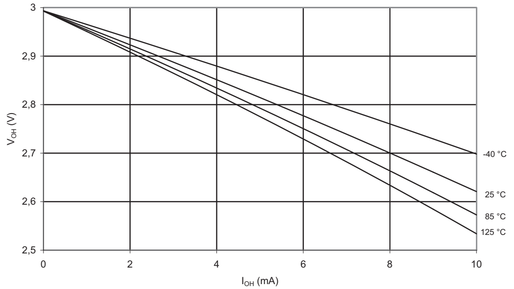
Figure 2-22. V_{OH} : Output Voltage vs. Source Current (I/O Pin, V_{CC} = 5V )
