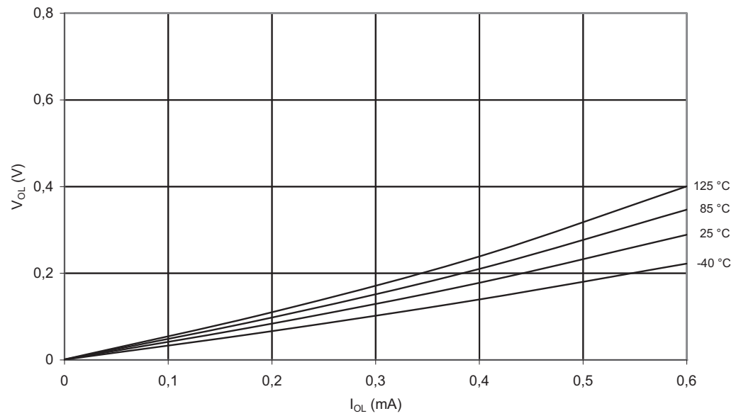
Figure 2-24. V_{OL} : Output Voltage vs. Sink Current (Reset Pin as I/O, V_{CC} = 3V )
