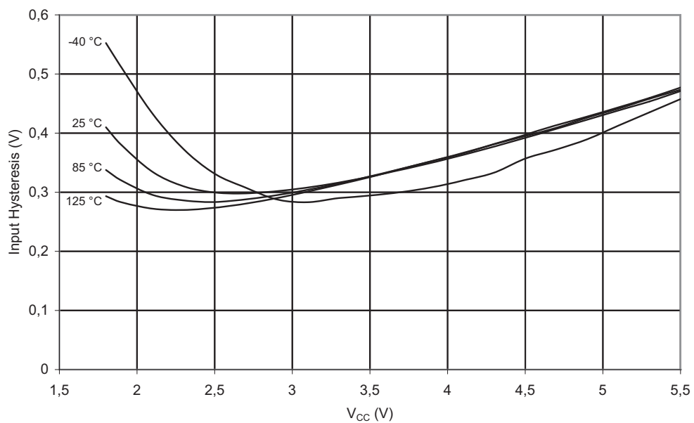
Figure 2-32. V_{IH} : Input Threshold Voltage vs. V_{CC} (Reset Pin, Read as '1')
