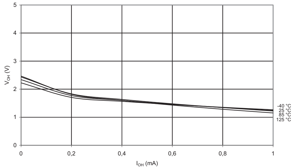
Figure 2-28. V_{OH} : Output Voltage vs. Source Current (Reset Pin as I/O, V_{CC} = 5V )
