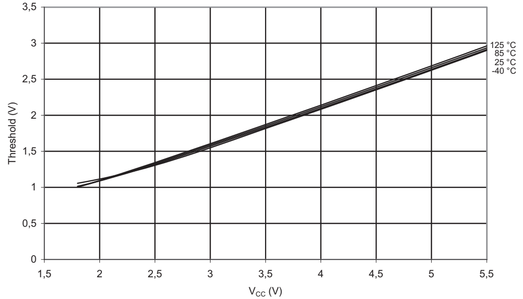
Figure 2-30. V_{IL} : Input Threshold Voltage vs. V_{CC} (I/O Pin, Read as '0')
