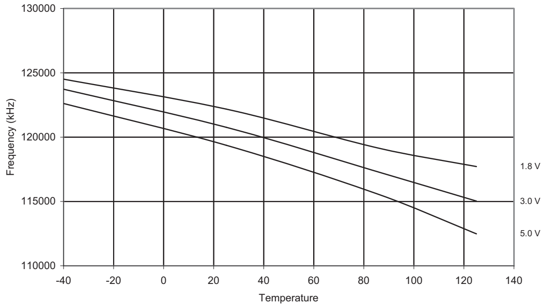
Figure 2-42. Frequency of Calibrated 8.0 MHz Oscillator vs. V_{CC}
