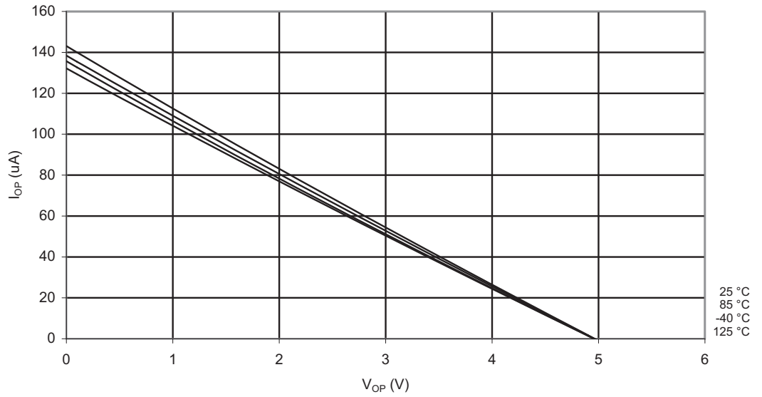
Figure 2-14. Pull-Up Resistor Current vs. Input Voltage (Reset Pin, V_{CC} = 1.8V )
