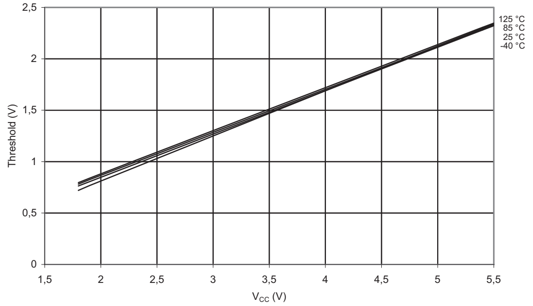
Figure 2-34. V_{IH}-V_{IL} : Input Hysteresis vs. V_{CC} (Reset Pin)
