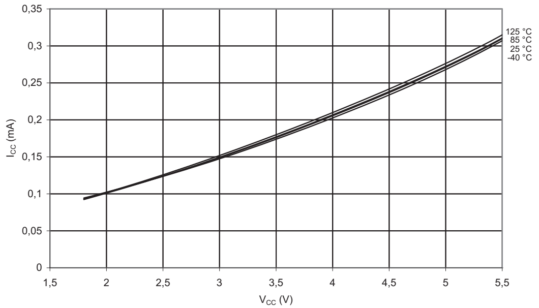
Figure 2-6. Idle Supply Current vs. V_{CC} (Internal Calibrated Oscillator, 128 kHz)
