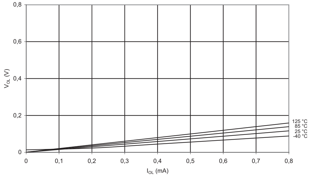
Figure 2-26. V_{OH} : Output Voltage vs. Source Current (Reset Pin as I/O, V_{CC} = 1.8V )
