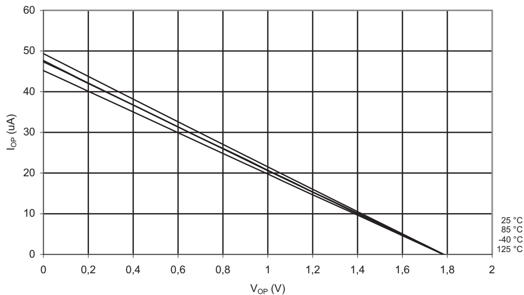
Figure 2-12. Pull-Up Resistor Current vs. Input Voltage (I/O Pin, V_{CC} = 2.7V )
