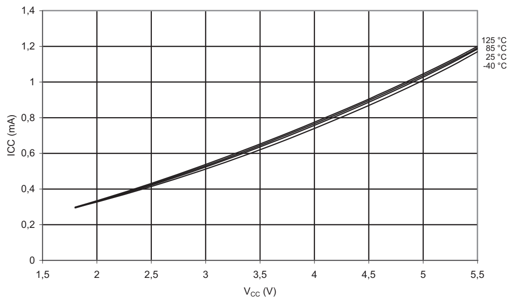
Figure 2-4. Idle Supply Current vs. V_{CC} (Internal Calibrated Oscillator, 8 MHz)
