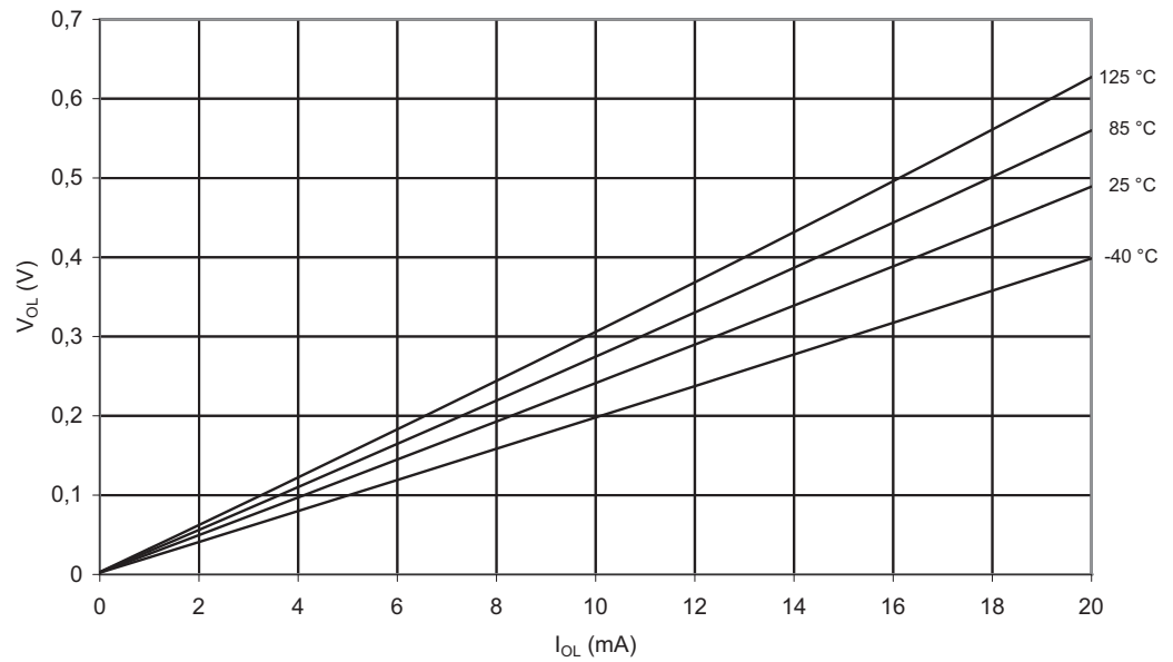
Figure 2-20. V_{OH} : Output Voltage vs. Source Current (I/O Pin, V_{CC} = 1.8V )
