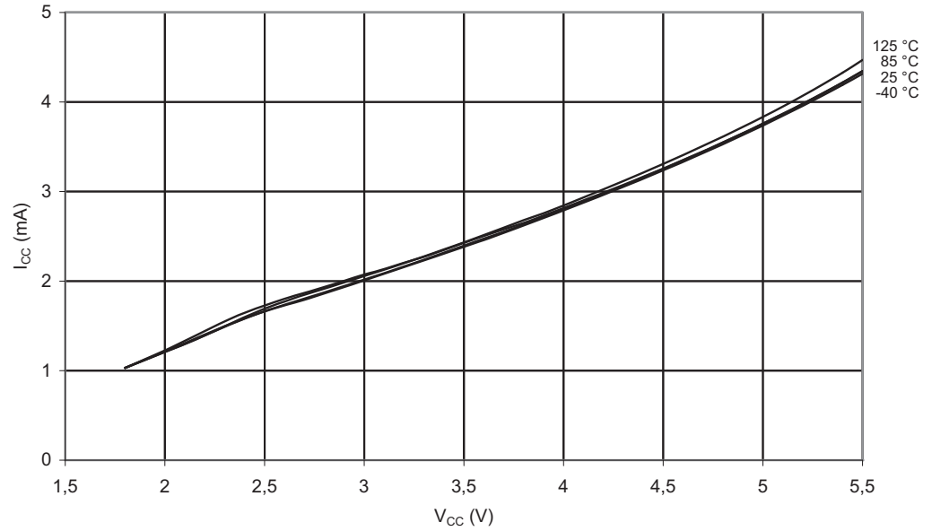
Figure 2-2. Active Supply Current vs. V_{CC} (Internal Calibrated Oscillator, 1 MHz)
