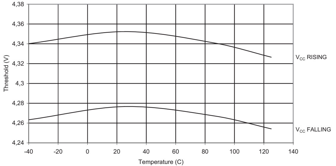
Figure 2-36. BOD Threshold vs. Temperature (BOD Level set to 2.7V)
