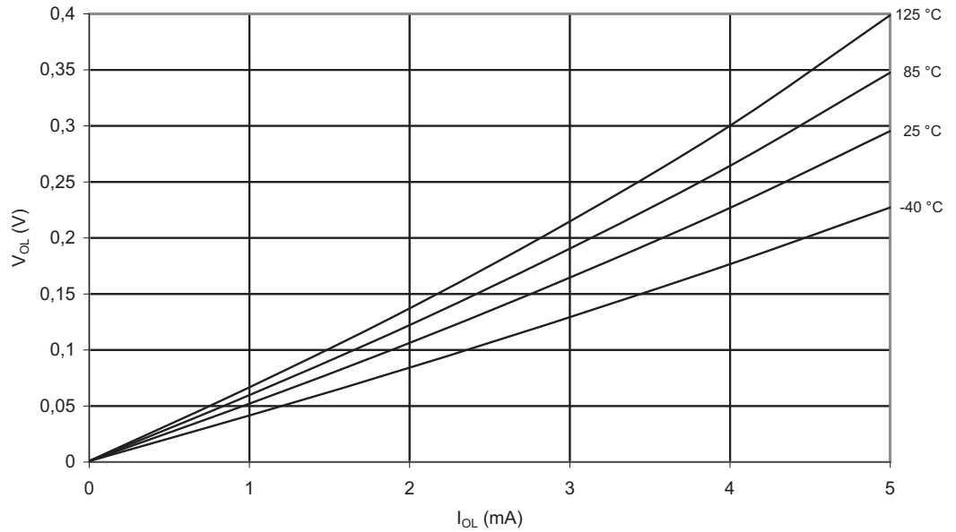
Figure 2-18. V_{OL} : Output Voltage vs. Sink Current (I/O Pin, V_{CC} = 3V )
