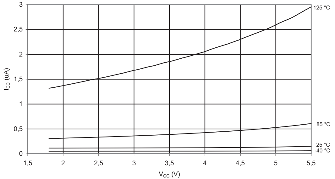
Figure 2-8. Power-down Supply Current vs. V_{CC} (Watchdog Timer Enabled)
