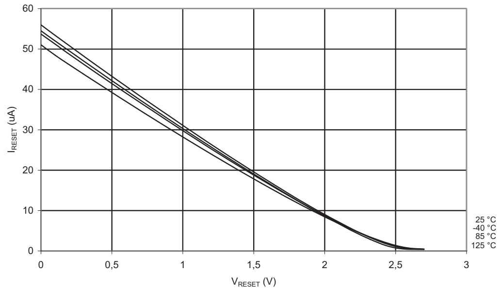
Figure 2-16. Pull-Up Resistor Current vs. Input Voltage (Reset Pin, V_{CC} = 5V )
