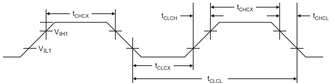
Figure 1-2. External Clock Drive Waveform
