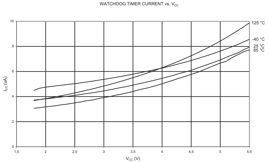
Figure 2-40. Watchdog Timer Current vs. V_{CC}
