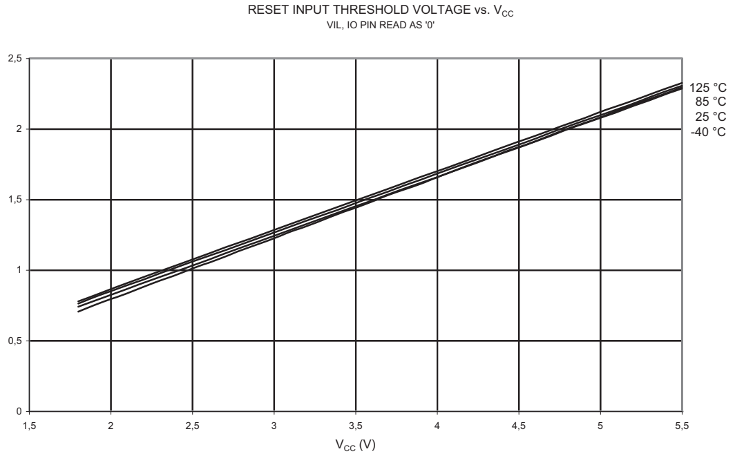
Figure 2-28. Reset Input Threshold Voltage vs. V_{CC} ( V_{IL} , I/O pin Read as '0')
