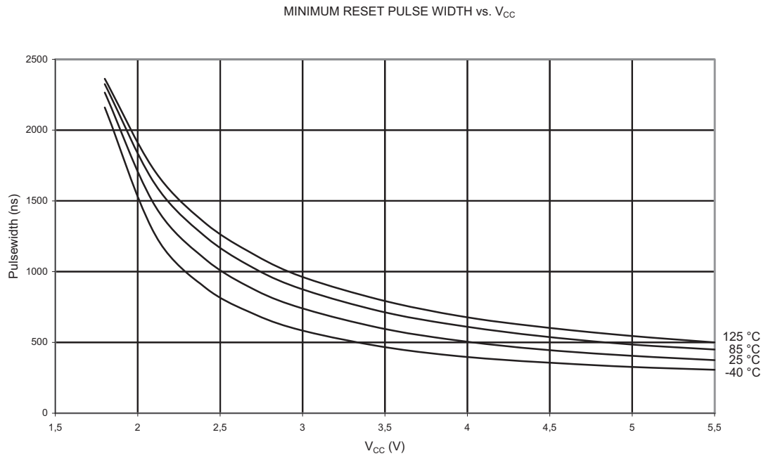
Figure 2-41. Minimum Reset Pulse Width vs. V_{CC}
