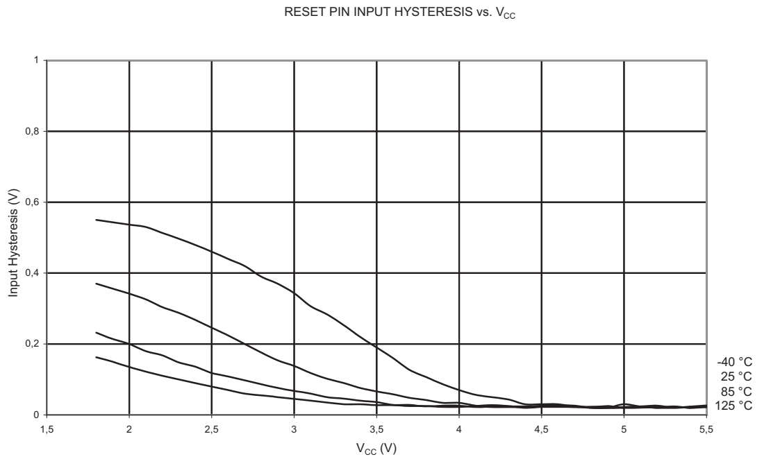
Figure 2-29. Reset Pin, Input Hysteresis vs. V_{CC}
