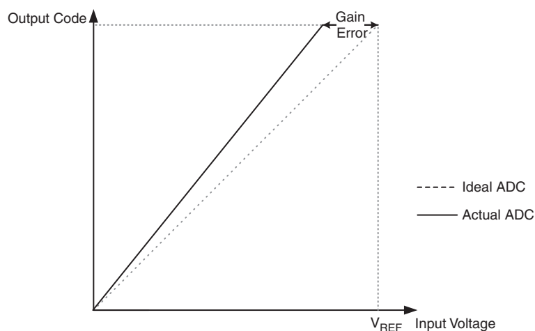
Figure 23-11. Gain Error
