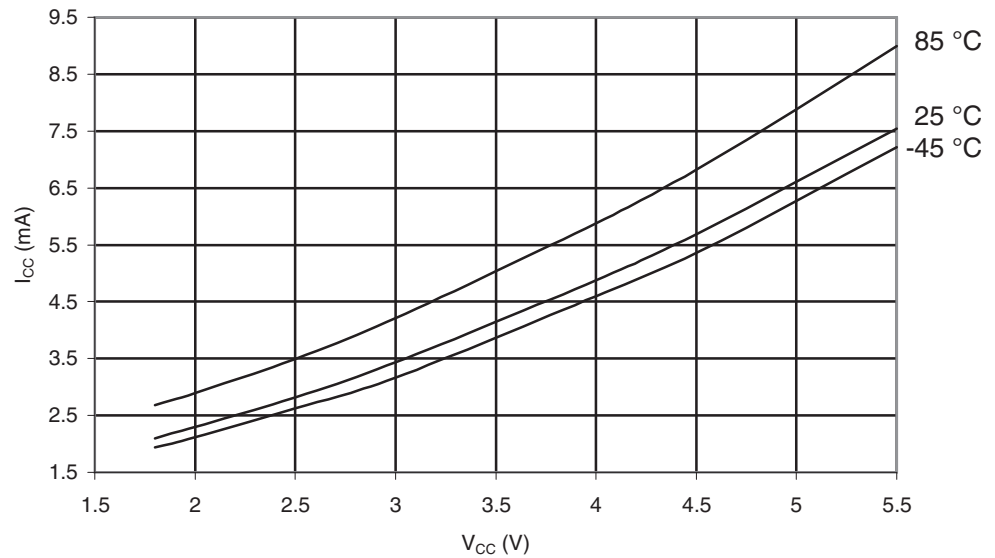
Figure 29-435. ATmega645P: Idle Supply Current vs. V_{CC} (32kHz Watch Crystal)
