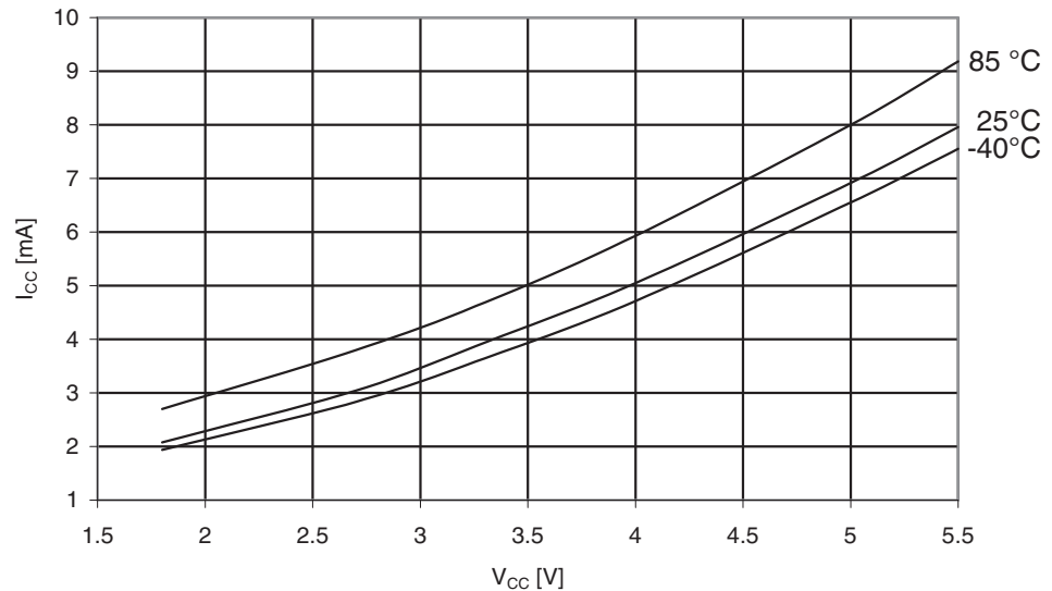
Figure 29-254. ATmega3250A: Idle Supply Current vs. V_{CC} (32kHz Watch Crystal)
