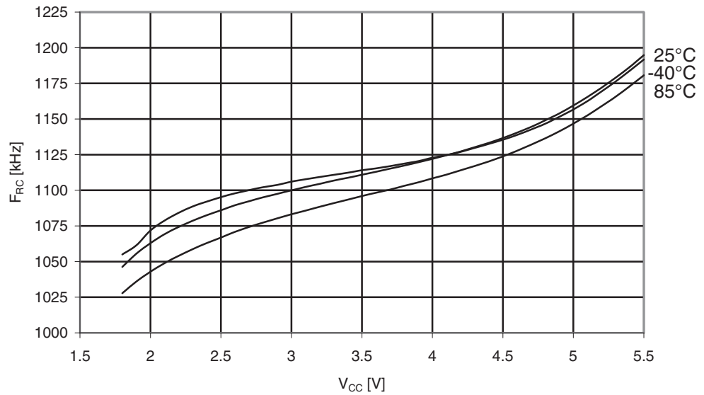
Figure 29-349. ATmega3250PA: Watchdog Oscillator Frequency vs. V_{CC}
