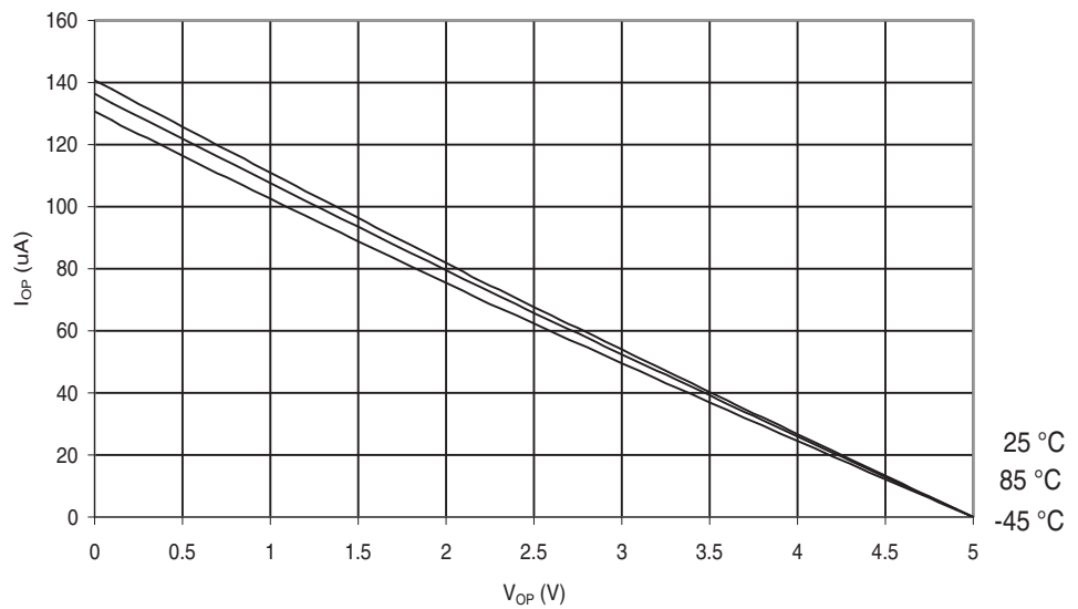
Figure 29-564. ATmega6450A: I/O Pin Pull-up Resistor Current vs. Input Voltage ( V_{CC} = 5V )
