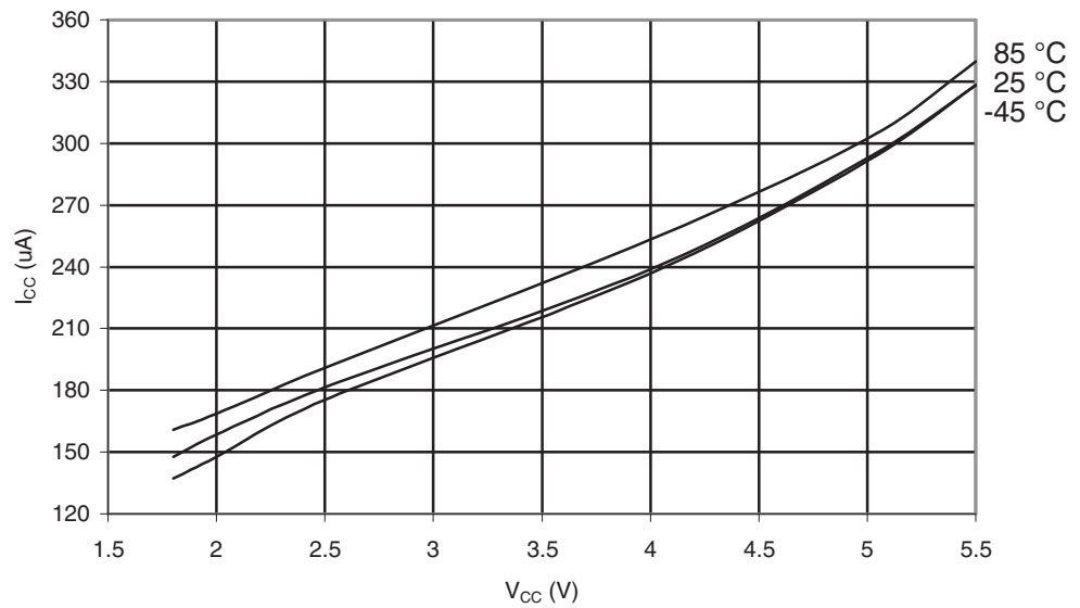
Figure 29-539. ATmega645P: Active Supply Current with ADC at 200kHz vs. V_{CC}
