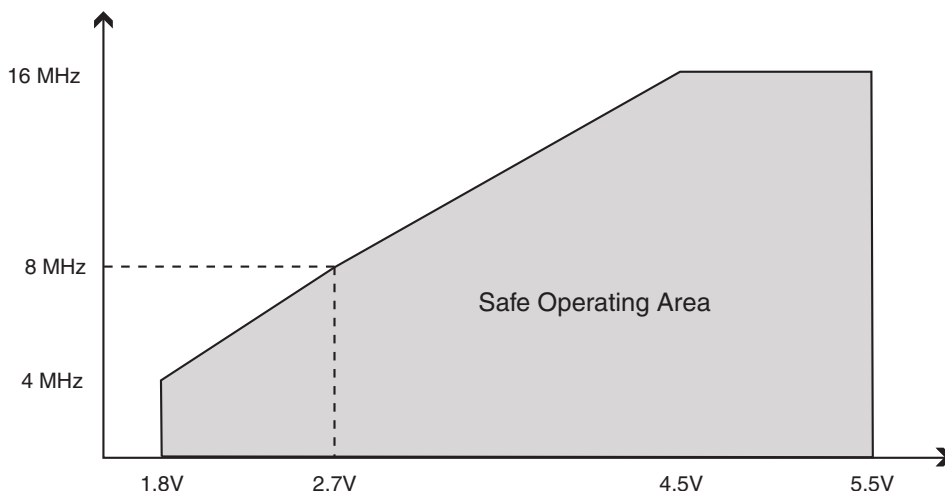
Figure 28-1. Maximum Frequency vs. V_{CC} , ATmega165A/165PA/ATmega645A/ATmega645P
