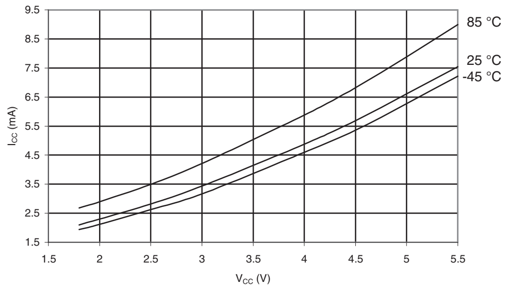
Figure 29-374. ATmega645A: Idle Supply Current vs. V_{CC} (32kHz Watch Crystal)
