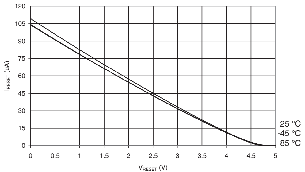
Figure 29-445. ATmega645P: Reset Pull-up Resistor Current vs. Reset Pin Voltage ( V_{CC} = 5V )
