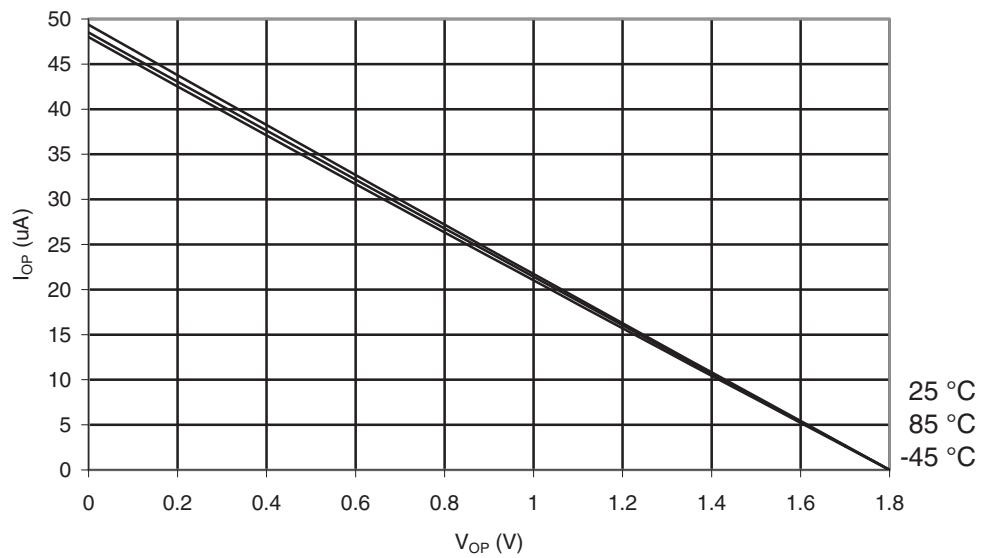
Figure 29-18. ATmega165A: I/O Pin Pull-up Resistor Current vs. Input Voltage ( V_{CC} = 1.8V )
