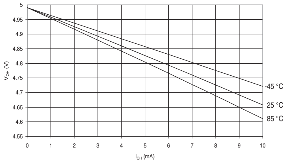
Figure 29-509. ATmega6450A: I/O Pin Output Voltage vs. Source Current, Ports A, C, D, E, F, G ( V_{CC} = 5V )
