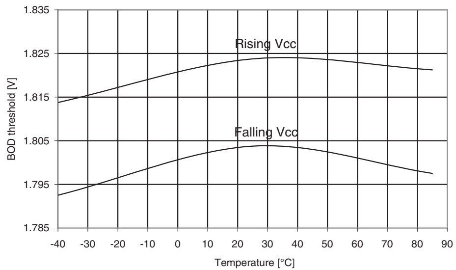
Figure 29-226. ATmega325PA: BOD Thresholds vs. Temperature (BOD Level is 1.8V)
