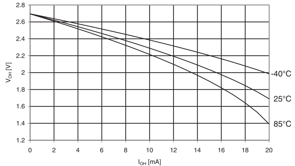
Figure 29-150. ATmega325A: I/O Pin Output Voltage vs. Source Current, Port B ( V_{CC} = 2.7V )
