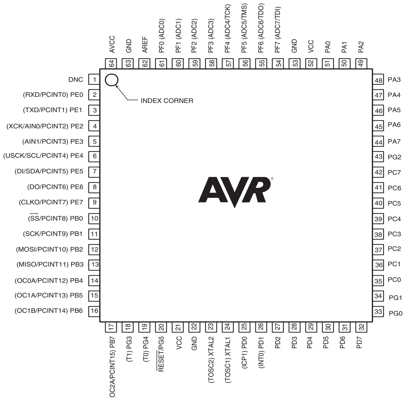
Figure 1-1. 64A (TQFP) and 64M1 (QFN/MLF) Pinout ATmega165A/ATmega165PA/ATmega325A/ATmega325PA/ATmega645A/ATmega645P
