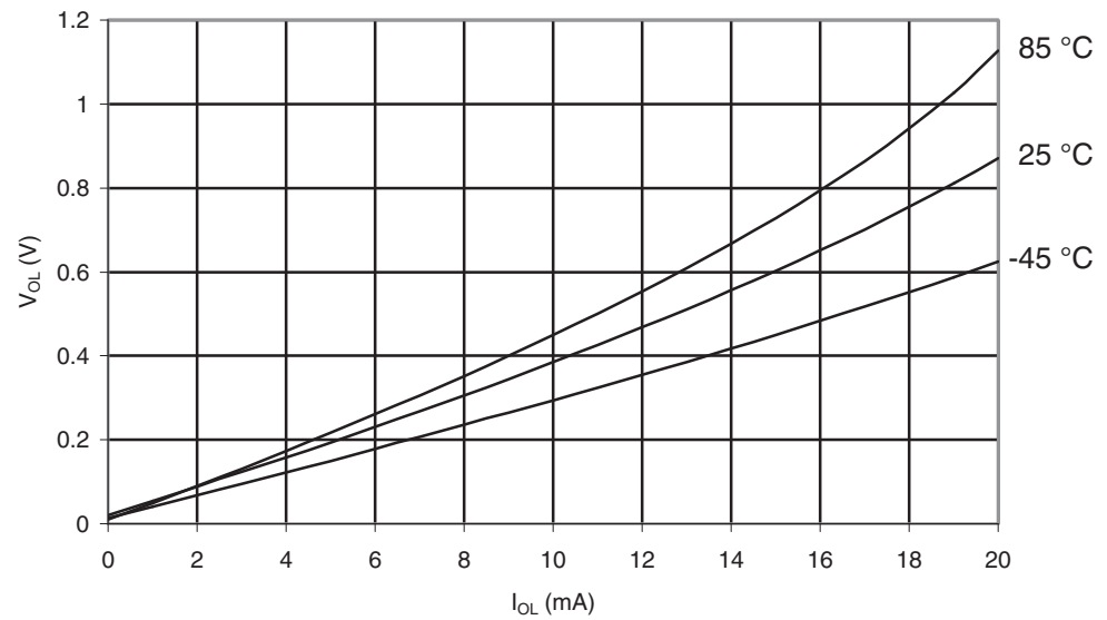
Figure 29-458. ATmega645P: I/O Pin Output Voltage vs. Sink Current, Port B ( V_{CC} = 2.7V )
