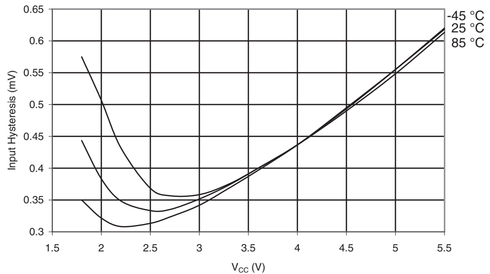
Figure 29-98. ATmega165PA: I/O Pin Input Hysteresis vs. V_{CC}
