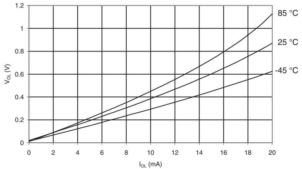
Figure 29-397. ATmega645A: I/O Pin Output Voltage vs. Sink Current, Port B ( V_{CC} = 2.7V )
