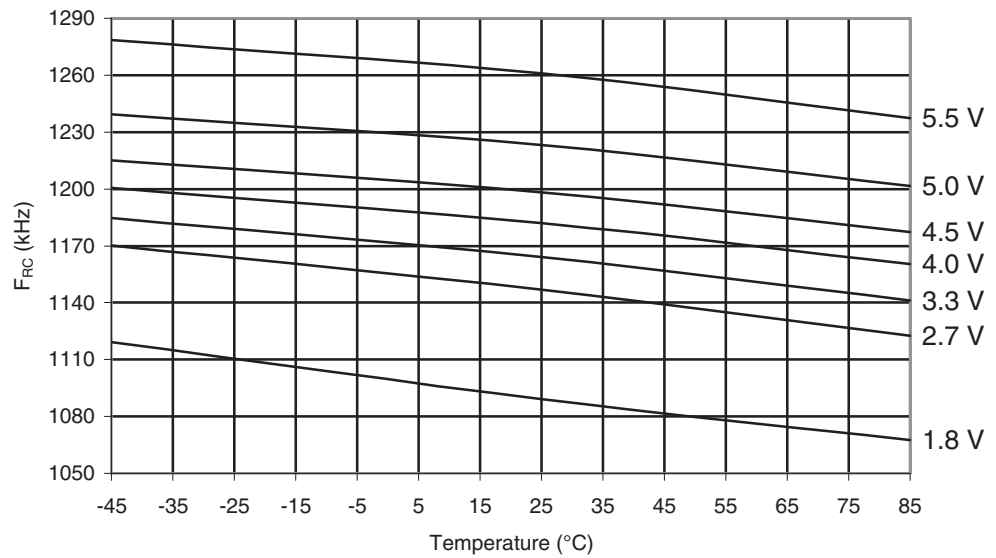
Figure 29-533. ATmega6450A: Watchdog Oscillator Frequency vs. Temperature
