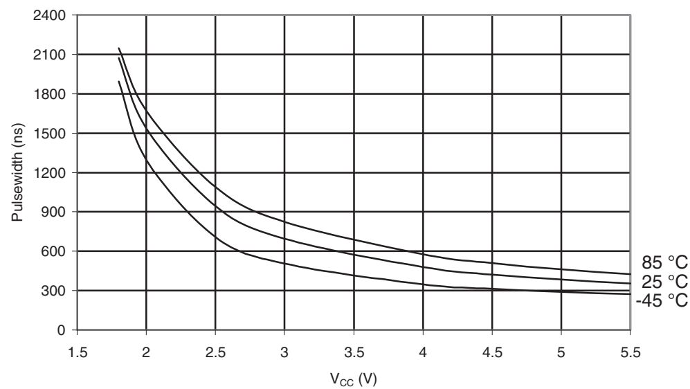
Figure 29-608. ATmega6450P: Minimum Reset Pulse Width vs. V_{CC}
