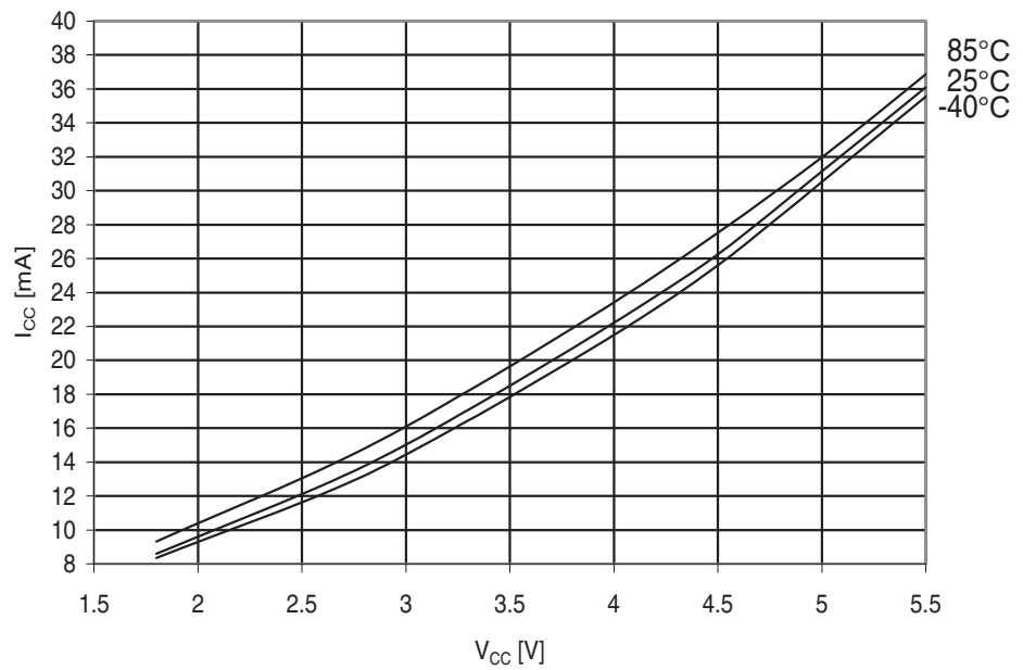
Figure 29-249. ATmega3250A: Active Supply Current vs. V_{CC} (32kHz Watch Crystal)
