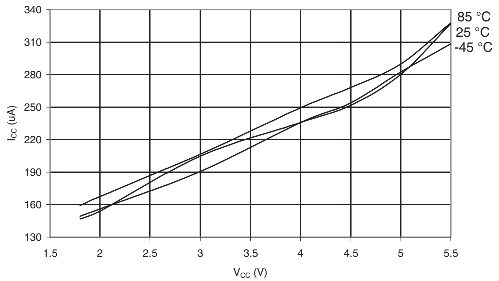
Figure 29-540. ATmega6450A: Active Supply Current with ADC at 1MHz vs. V_{CC}
