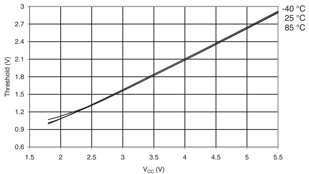
Figure 29-218. ATmega325PA: I/O Pin Input Threshold Voltage vs. V_{CC} ( V_{IH} , I/O Pin Read as "1")
