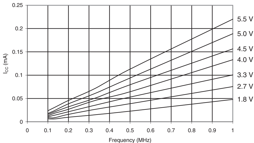
Figure 29-1. ATmega165A: Active Supply Current vs. Frequency (0.1 - 1.0MHz)
