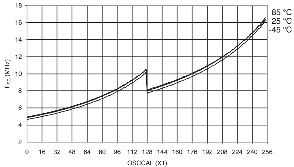
Figure 29-597. ATmega6450P: Calibrated 8MHz RC Oscillator Frequency vs. Oscal Value
