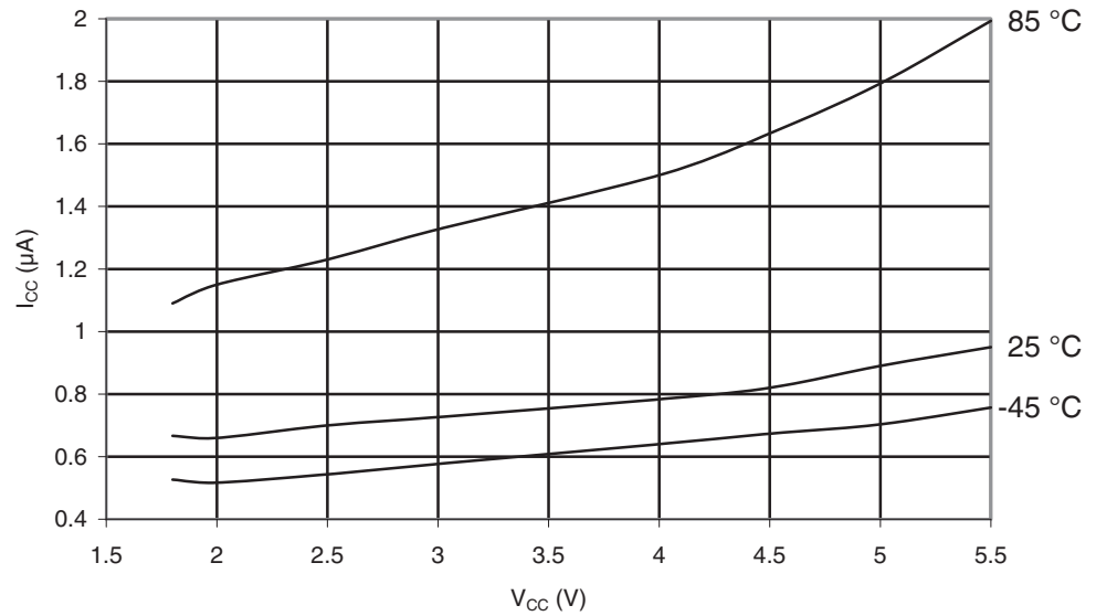
Figure 29-15. ATmega165A: Standby Supply Current vs. V_{CC} (Xtall and Resonator, Watchdog Timer Disabled)
