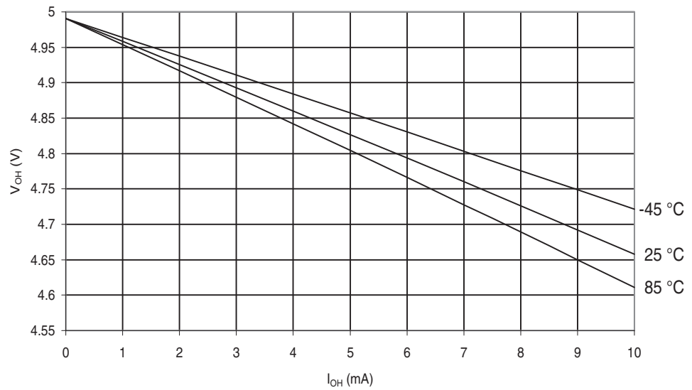
Figure 29-387. ATmega645A: I/O Pin Output Voltage vs. Source Current, Ports A, C, D, E, F, G ( V_{CC} = 5V )
