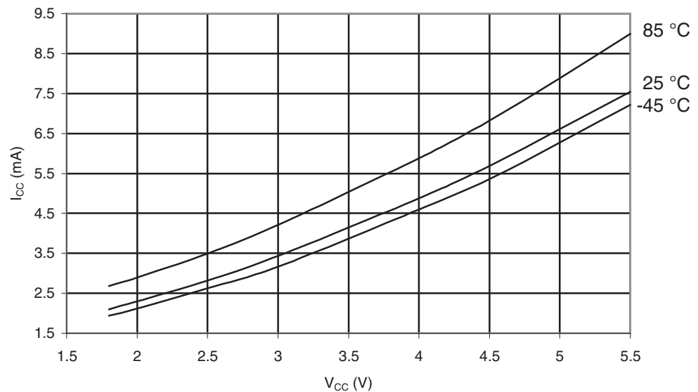
Figure 29-557. ATmega6450A: Idle Supply Current vs. V_{CC} (32kHz Watch Crystal)
