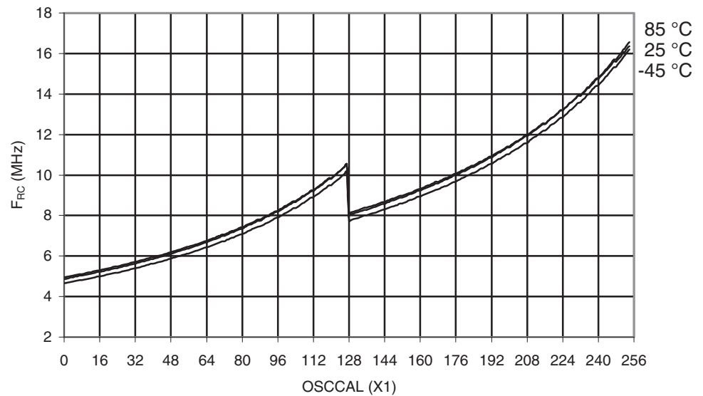
Figure 29-475. ATmega645P: Calibrated 8MHz RC Oscillator Frequency vs. Oscscal Value
