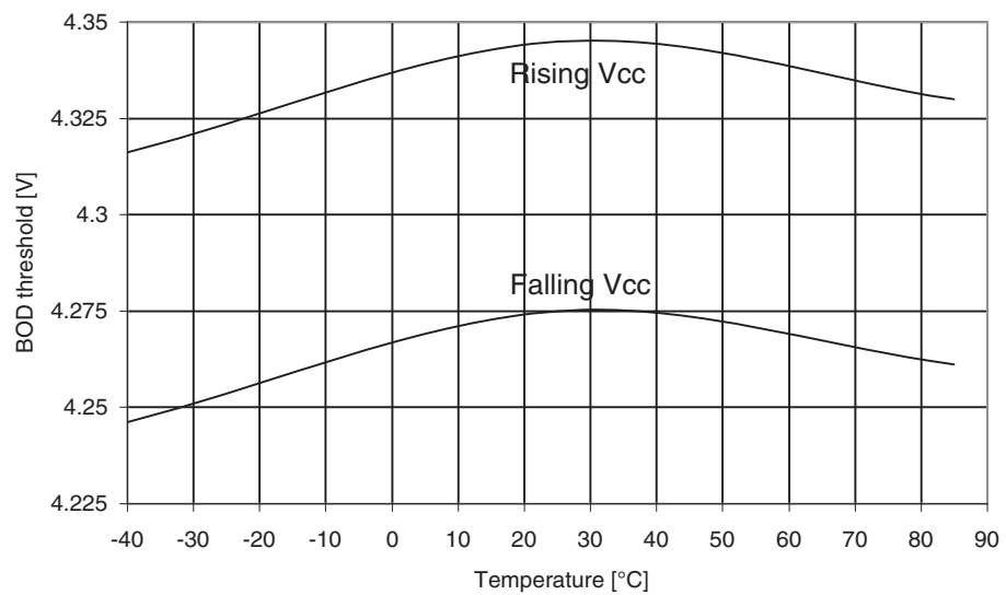
Figure 29-284. ATmega3250A: BOD Thresholds vs. Temperature (BOD Level is 4.3V)
