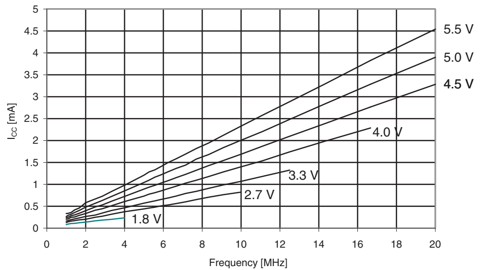
Figure 29-131. ATmega325A: Idle Supply Current vs. Frequency (1 - 20MHz)
