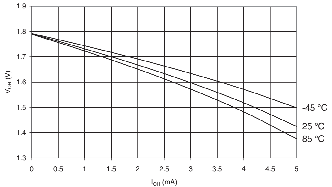
Figure 29-89. ATmega165PA: I/O Pin Output Voltage vs. Source Current, Port B ( V_{CC} = 1.8V )
