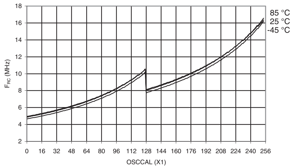
Figure 29-414. ATmega645A: Calibrated 8MHz RC Oscillator Frequency vs. Oscscal Value
