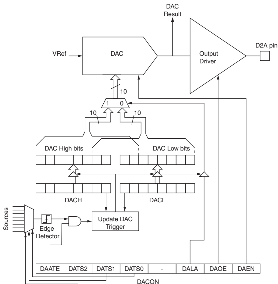
Figure 22-1. Digital to Analog Converter Block Schematic
