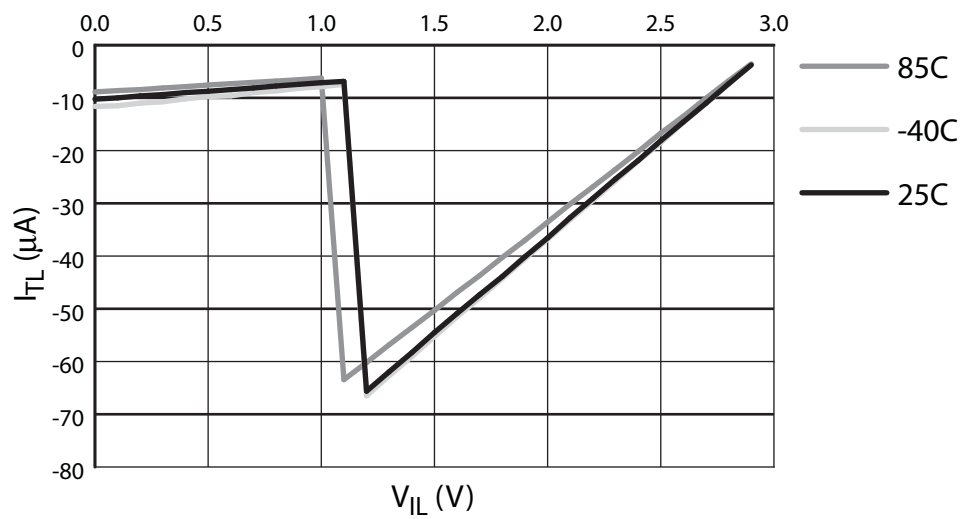
Figure 18-6. Quasi-bidirectional Input Transition Current at 3V
