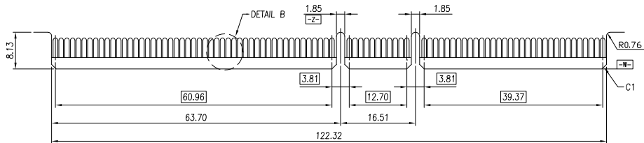
RECOMMENDED MATING COMPONENT BOARD (5.0V) Tolerance: ±0.05
