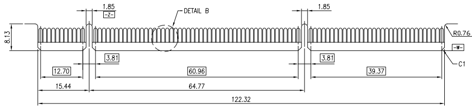
RECOMMENDED MATING COMPONENT BOARD (3.3V) Tolerance: ±0.05
