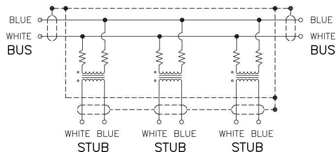
THREE STUB COUPLER SCHEMATIC
