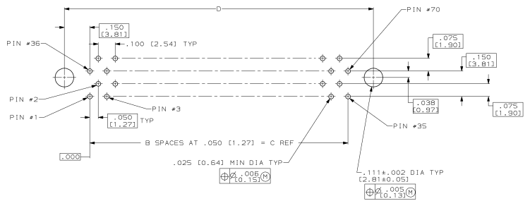
RECOMMENDED P.C. BOARD HOLE PATTERN (CONNECTOR SIDE)
