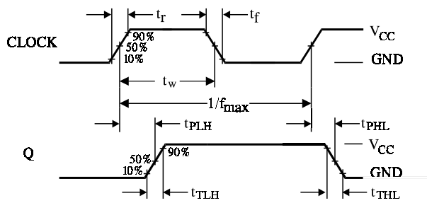
Figure 1. Switching Waveforms
