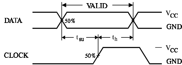
Figure 3. Switching Waveforms
