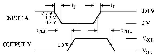
Figure 1. Switching Waveforms
