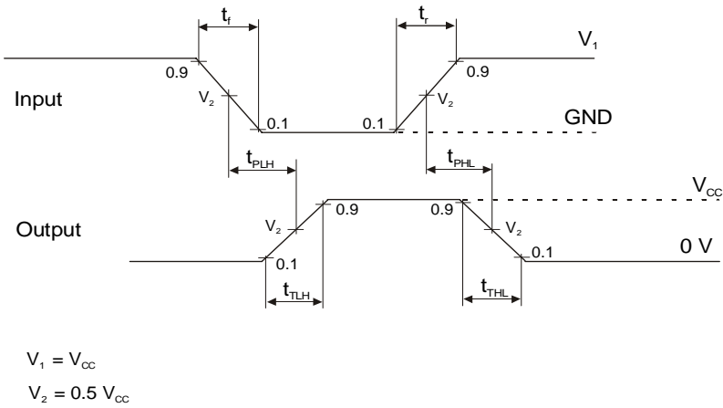
Figure 1. Switching Waveforms
