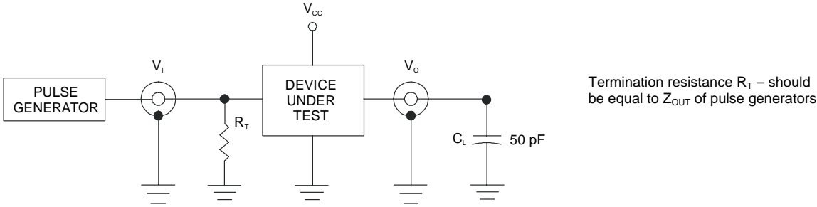
Figure 2. Test Circuit
