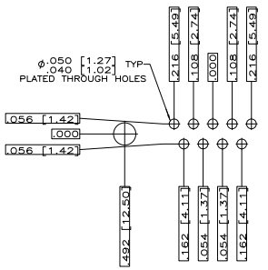
RECOMMENDED P.C. BOARD LAYOUT SHELL SIZE 1 (9 POSITION) Δ
