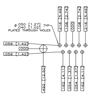
RECOMMENDED P.C. BOARD LAYOUT SHELL SIZE 1 (9 POSITION)
