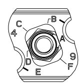
JACKSCREW POLARIZATION "A" SHOWN SCALE 4:1
