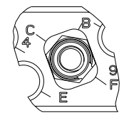
JACKSCREW POLARIZATION "F" SHOWN SCALE 4:1
