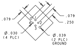
PCB LAYOUT 1738916-1, 2, AND 3
